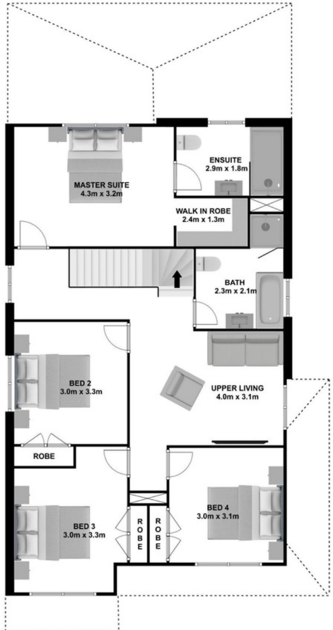
FIRST FLOOR
