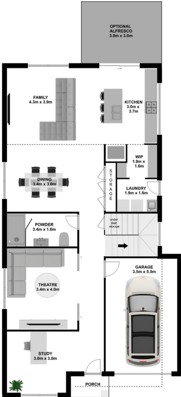
GROUND FLOOR
